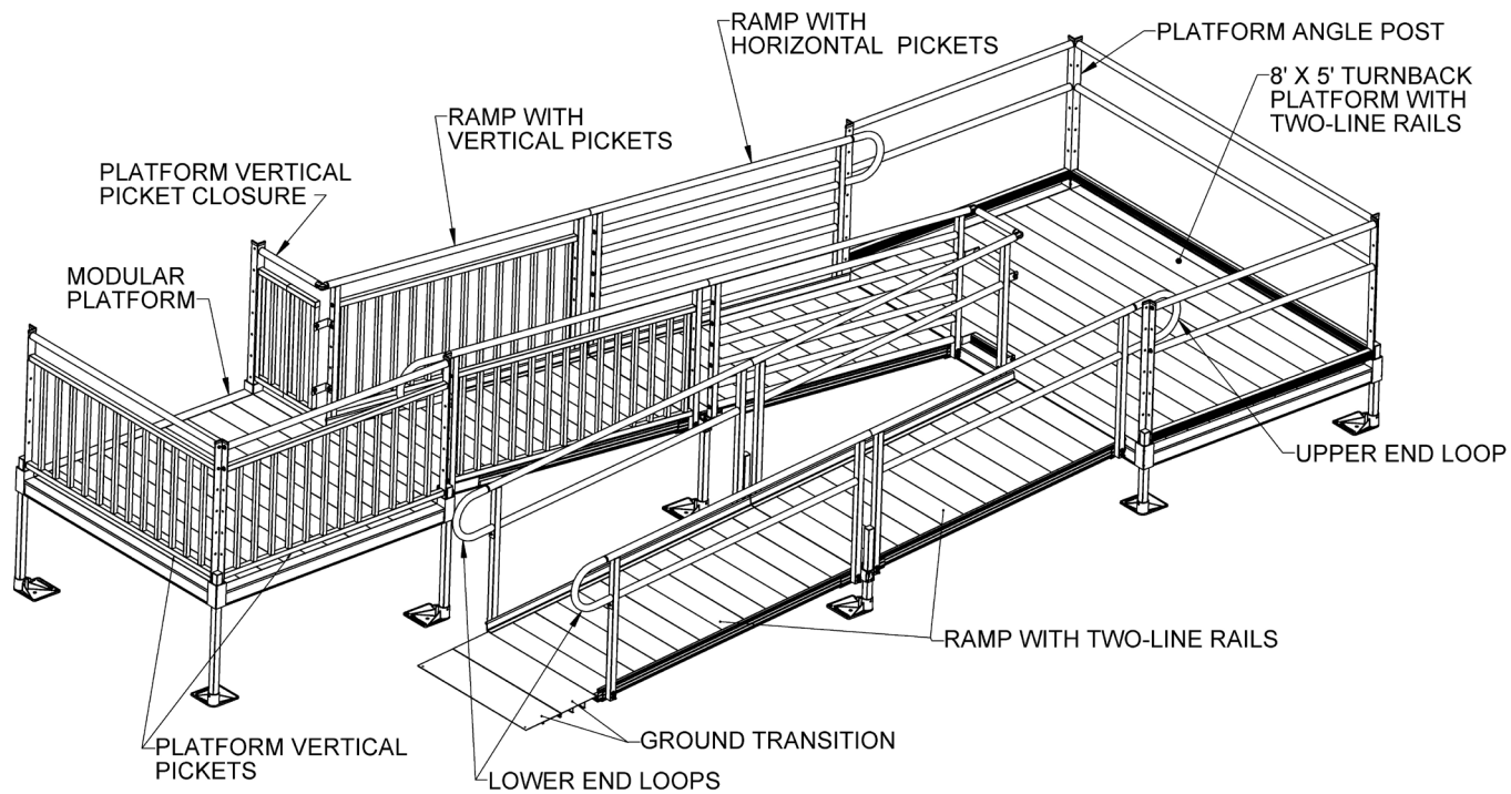
ISOMETRIC VIEW
